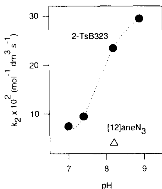
Figure 5. Second-order rate constants of PNPA hydrolysis as a function of pH with the Zn.8 complex.
