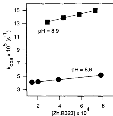
Figure 1. Acceleration of PNPA hydrolysis in the presence of Zn. B323 complexes.
