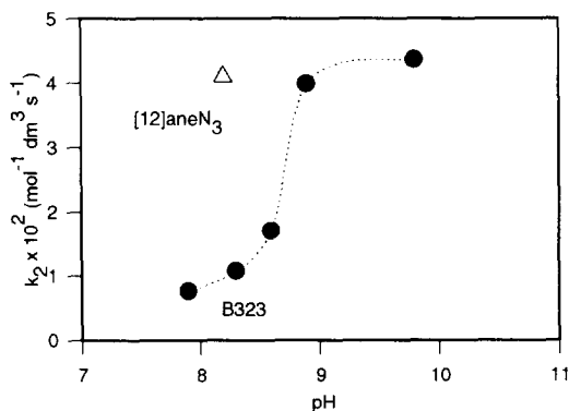
Figure 2. Second order rate constants of PNPA hydrolysis as a function of pH with the Zn. B323 complex.
