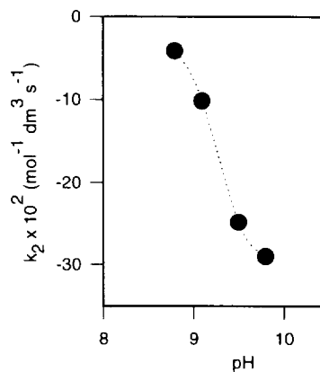
Figure 4. Second-order rate constants of PNPA hydrolysis as a function of \text{pH} with the \text{Zn} \cdot \mathbf{D323} complex.
