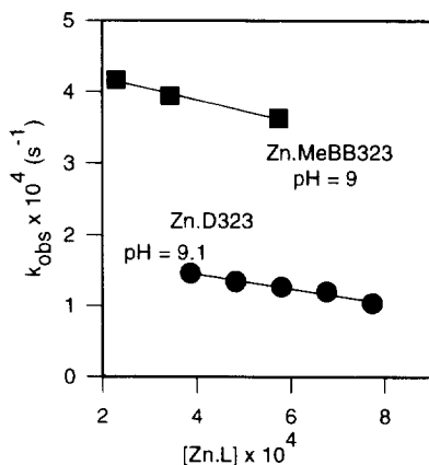
Figure 3. Inhibition of PNPA hydrolysis in the presence of the \text{Zn} \cdot \mathbf{4} complex ( \text{pH} = 9.1 ) and the \text{Zn} \cdot \mathbf{6} complex ( \text{pH} = 9.0 ).
